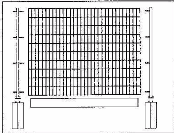
Type : D.F. 2000 Fence Height 1.95 m. Wire diameter 7x5.5 mm. Width 2.4 m. Spacing 200mm X 75 mm.
